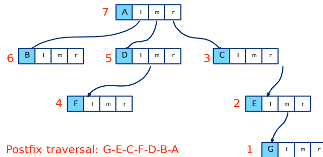
Figure 1: Postfix Traversal.
